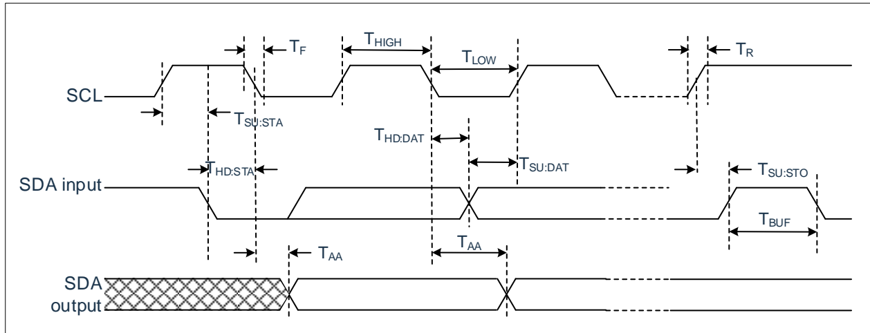
Figure 20-2: I²C™ Bus Data Timing
