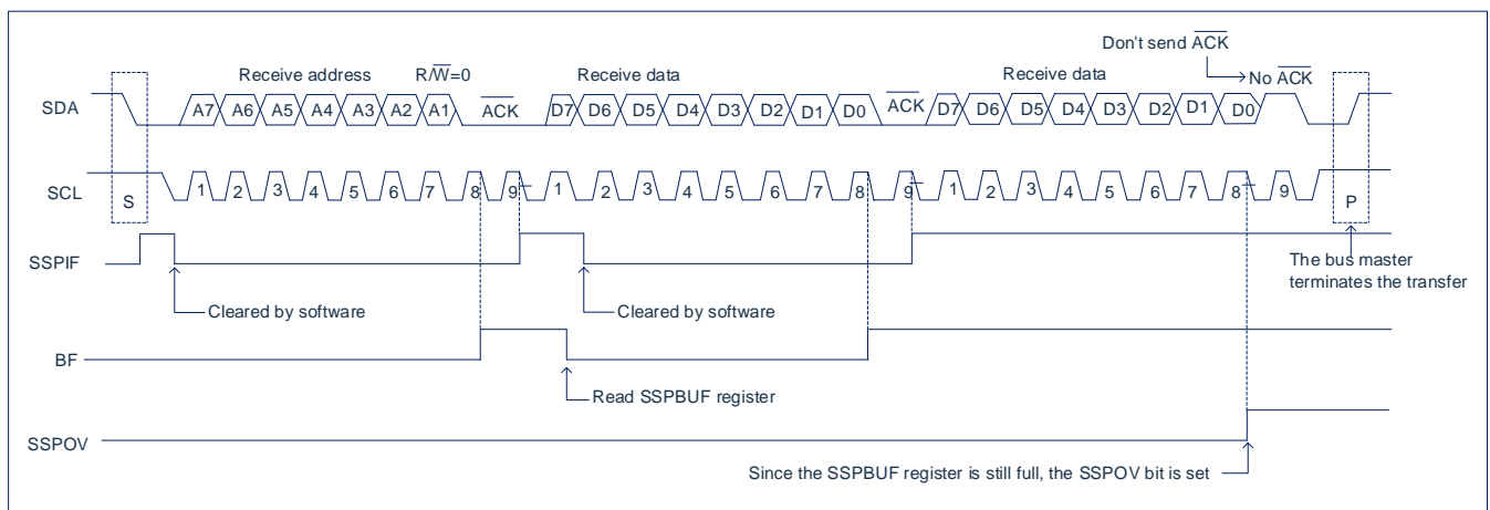
Fig 15-17: Time series for I 2 C™ slave mode receive (7-bit address)
