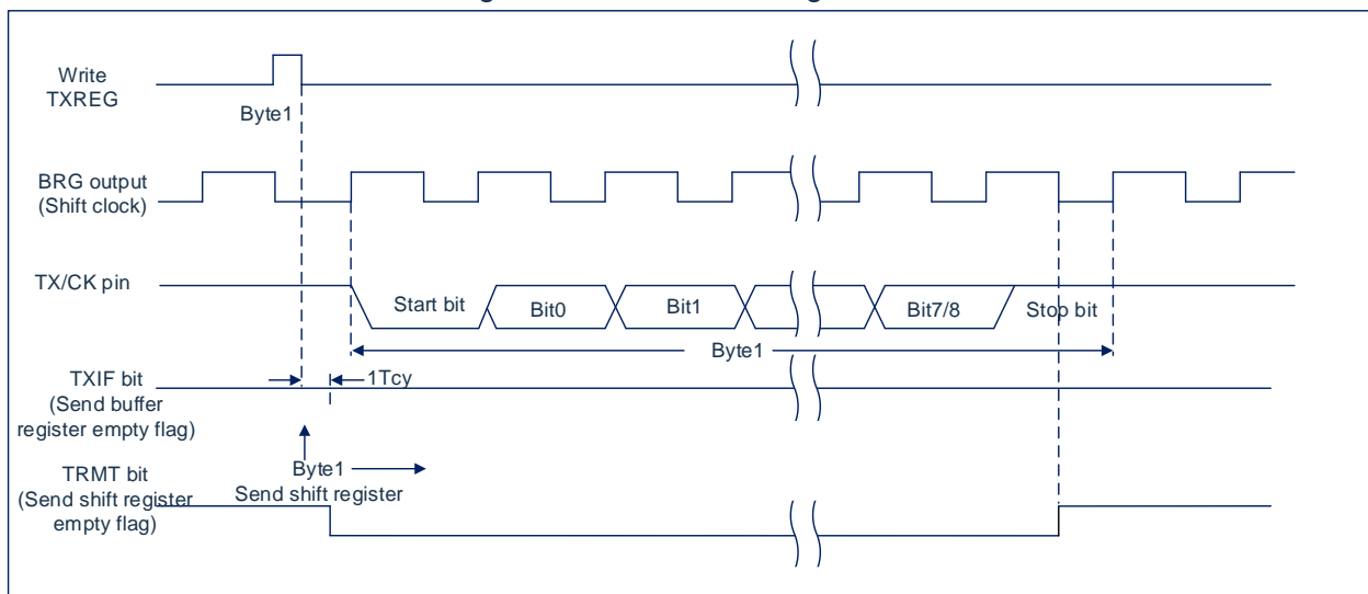
Fig 14-3: asynchronous transmit
